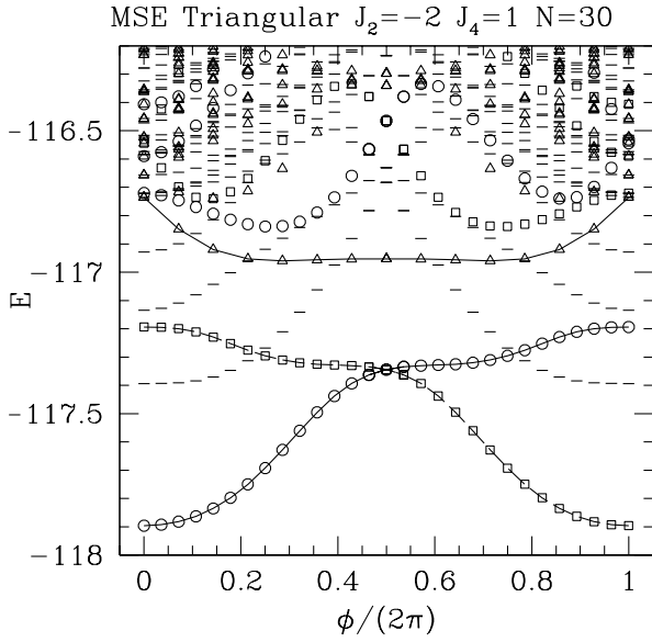
Fig. 8. Low-lying spectrum of the 6 \times 5 sample of the multiple-spin exchange model (Eq. (55)) as a function of the twist \phi at the x boundary of the sample. Same symbols as in Figure 4. On this small sample the lowest S_{\text{tot}}^z = 1 state is a |S^z = 1, \mathbf{k} = (2\pi/3, 0)\rangle . We suspect that in the thermodynamic limit the lowest S^z = 1 eigenstate has a wave-vector belonging to the star of (\pi/2, 0) (these wave-vectors are not allowed in the present sample).
