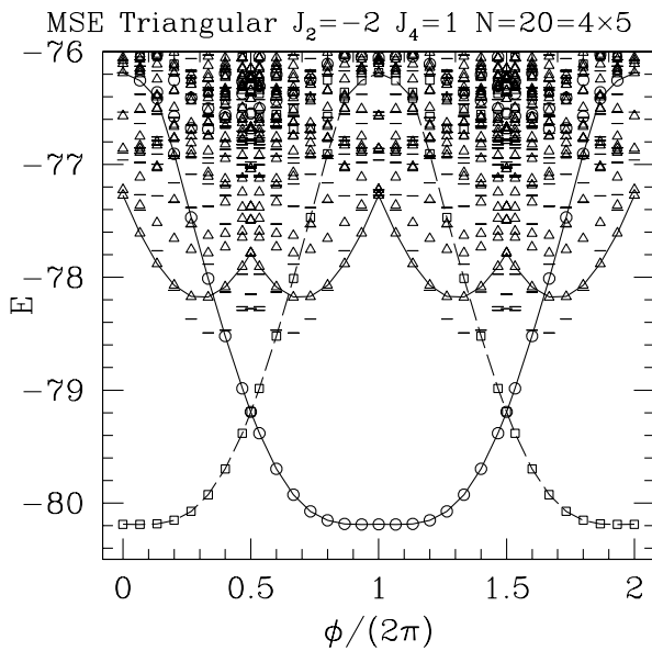
Fig. 5. Low-lying spectrum of the 4 \times 5 sample of the multiple-spin exchange model (Eq. (55)) as a function of the twist \phi at the x boundary of the sample. Same symbols as in Figure 4. We suspect that for this spin liquid, in the thermodynamic limit the wave vector of the first S_{\text{tot}}^z = 1 state is (\pi/2, 0) . But in the finite small samples that are available we never have this wave vector (except in the 4 \times 6 sample): this explains the discontinuities in the shape of the lowest S_{\text{tot}}^z = 1 state.
