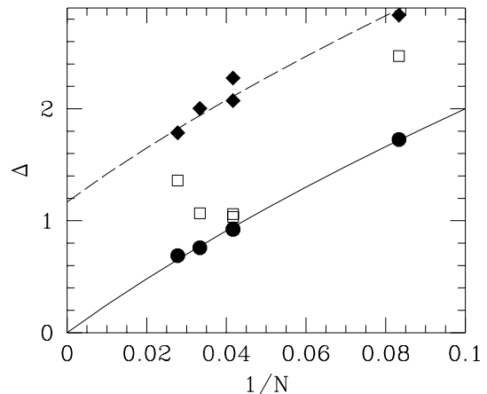
Fig. 2. Finite-size scaling of various gaps to excited states. Black circles: \Delta_s gap to the first S = 1 state (it has wave-vector W_{1(2)} in the Brillouin zone of Fig. 1). Open squares: \Delta_0 gap to the first |\pi, 0, S = 0\rangle state (points K_i in the Brillouin zone). Black diamonds: \Delta_1 gap to the first |\pi, 0, S = 1\rangle state.
