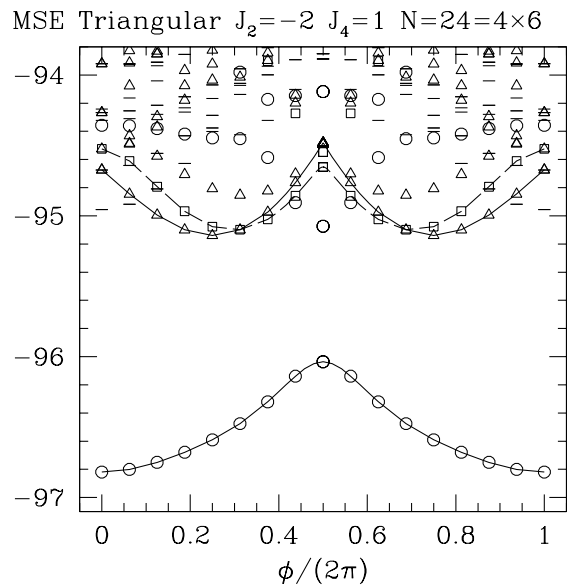
Fig. 6. Low-lying spectrum of the 4 \times 6 sample of the multiple-spin exchange model (Eq. (55)) as a function of the twist \phi at the x boundary of the sample. Same symbols as in Figure 4.
