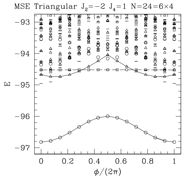
Fig. 7. Low-lying spectrum of the 6 \times 4 sample of the multiple-spin exchange model (Eq. (55)) as a function of the twist \phi at the x boundary of the sample. Same symbols as in Figure 4.
